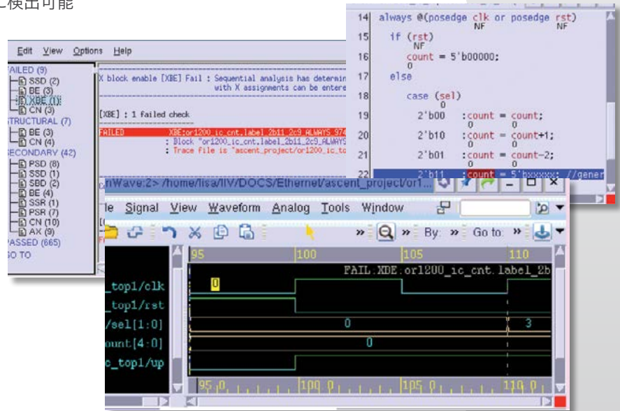
Figure 1. Debugging is fast and easy with cross probing to RTL design source and VCD waveform to pinpoint design issues.
